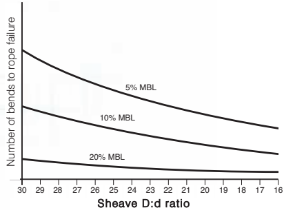
Effects of D:d Ratio and loading on fatigue life - Typical example Dyform 6
