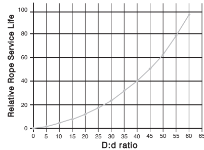
Service life curve for various D:d ratios
