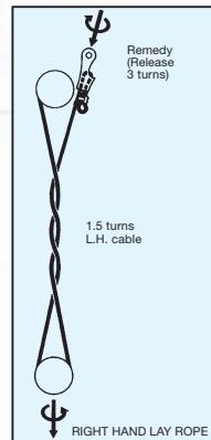
Fig 16 outboard anchorage. If left hand cabling is produced in the reeving system, correction is usually achieved (on the right hand lay ropes, see Fig. 16) by releasing turn at the anchorage. Effort must be made to work released or induced turn throughout the working length of rope, by operating the crane at maximum height of lift with a light load. It may be necessary to repeat the process until the cabling has been corrected. For right hand cable it will normally be necessary to induce turn at the anchorage.
