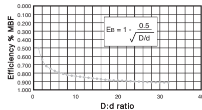
Approximate loss in breaking strength due to bending
